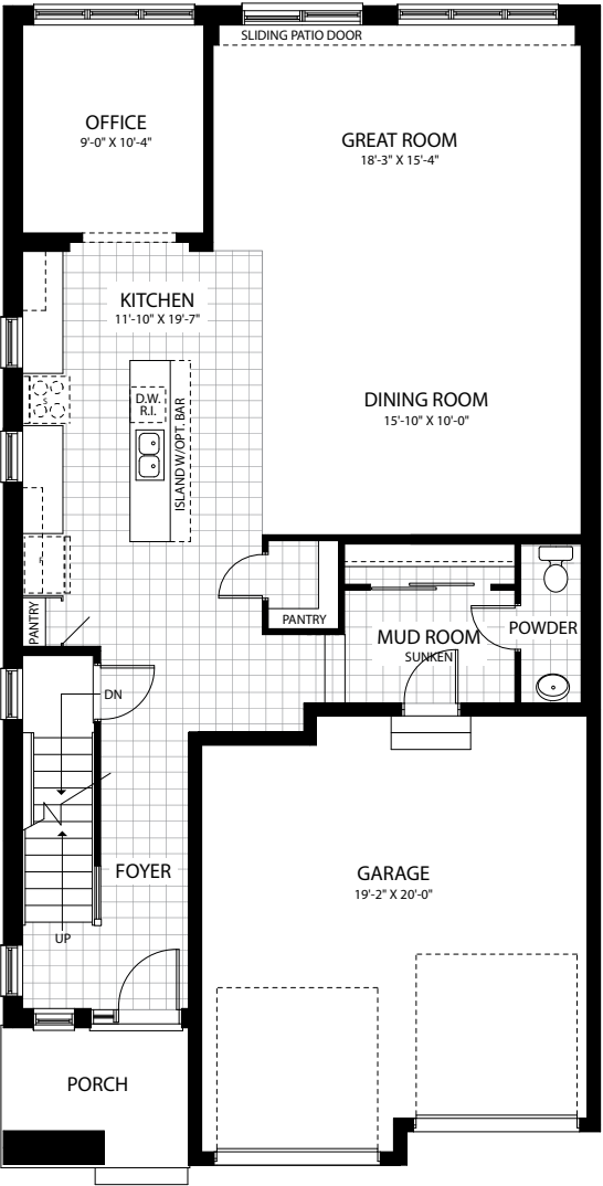
MAIN FLOOR 1208 SQ.FT.
