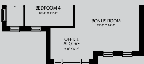
SECOND FLOOR - 1634 SQ.FT.
