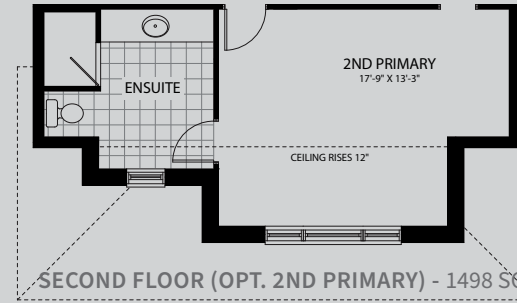
SECOND FLOOR 1498 SQ.FT.
