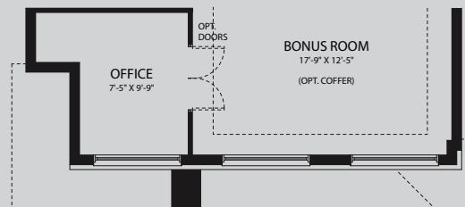
SECOND FLOOR - 1438 SQ.FT.
