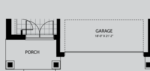
MAIN FLOOR - 1111 SQ.FT.
