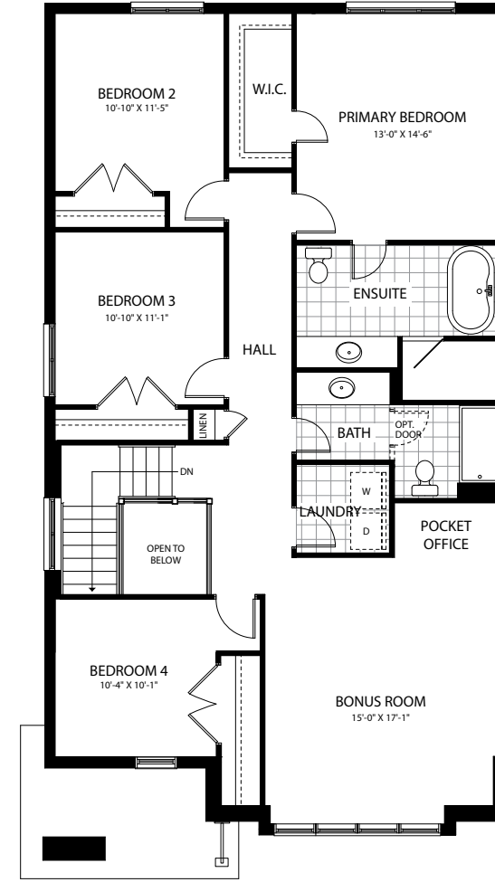
SECOND FLOOR 1498 SQ.FT.
