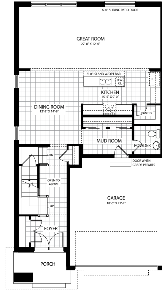
MAIN FLOOR 1111 SQ.FT.
