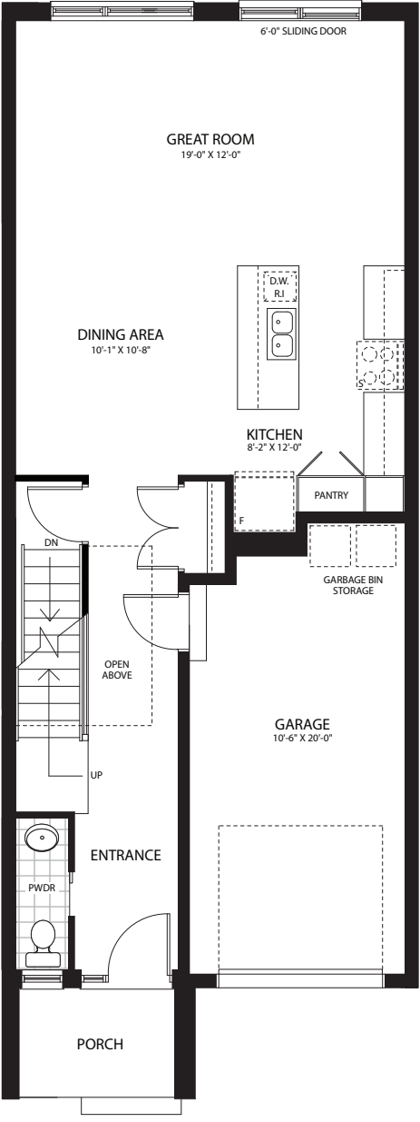
MAIN FLOOR 712 SQ.FT.
